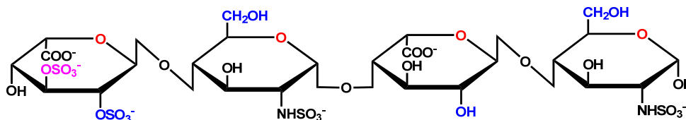
HS15a_3-O-SO3_HS15: GOLD Score 127
