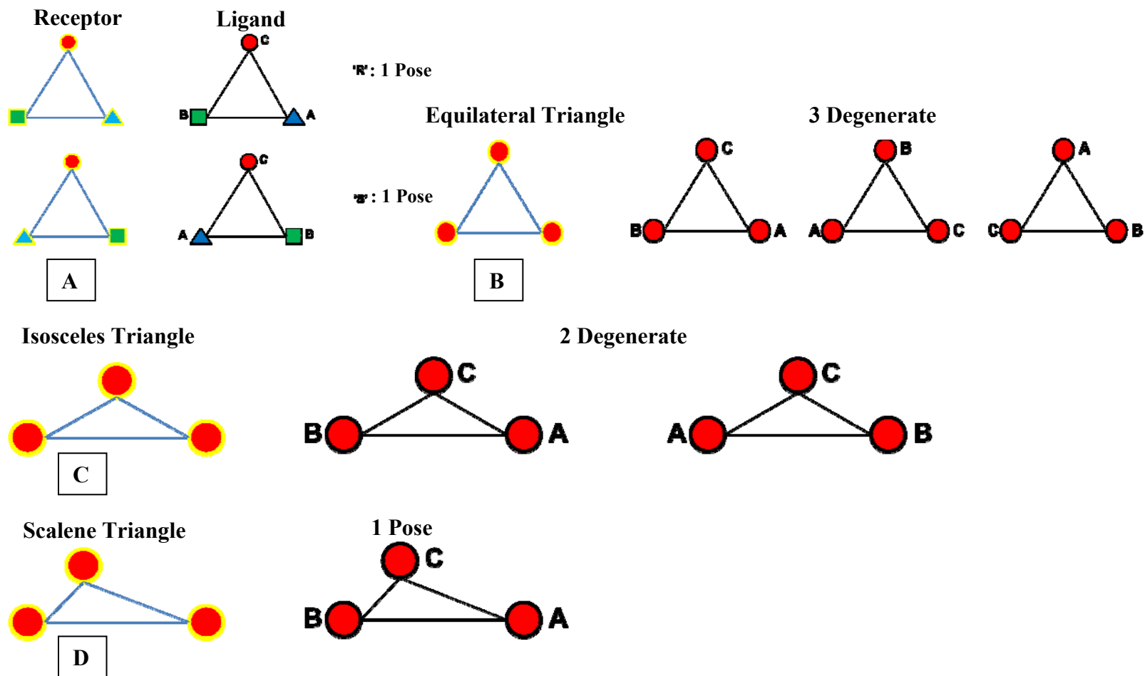
Figure 49b. A. Equilateral triangle receptor ('three-point pharmacophore') showing limited binding mode for the typical R - and S - isomer of tetrahedral ligands. Three substituents (represented by different shapes) are non-equivalent. B. Lys-sulfate or Arg-sulfate kind of non-directional interactions exhibit multiple binding modes in equilateral triangle receptor geometry. C. Isosceles and D. Scalene triangles show single binding mode.
