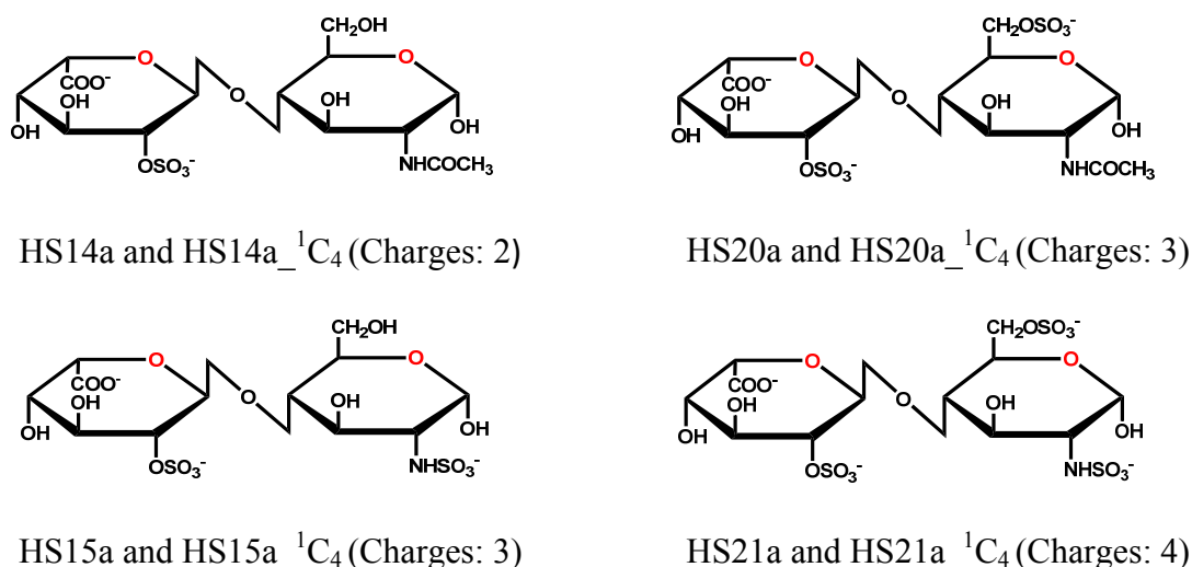
Figure 52. Building blocks for heparin oligomers used to build the octasaccharide library of 4096 sequences. Disaccharide units are named as HS+number+a where ‘a’ denotes an additional sulfate group at 2 nd position of the iduronic acid. Since iduronic acid can exist in {}^1C_4 or {}^2S_0 forms, a suffix {}^1C_4 is added. No suffix indicates {}^2S_0 conformation.
